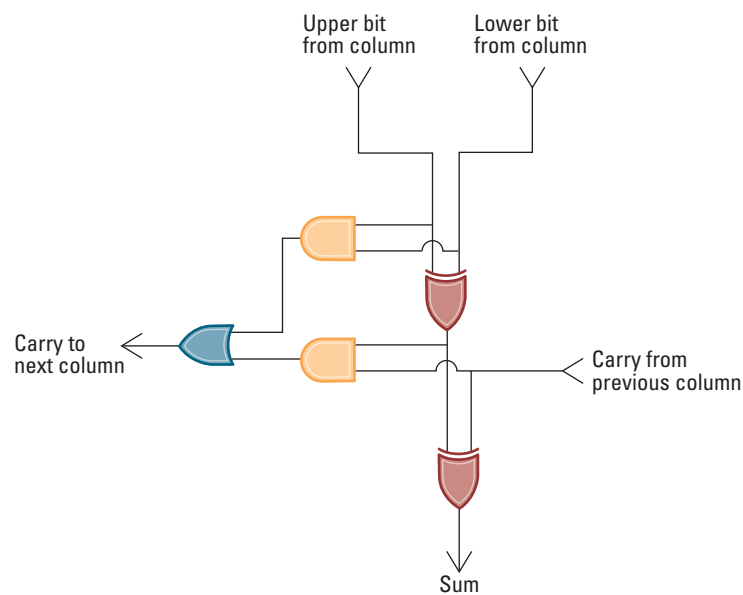
Figure B.2 A circuit to add a single column in a multiple-column addition problem
